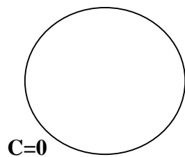
ELIPSE
