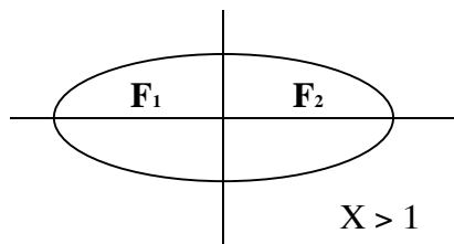
ELIPSE
